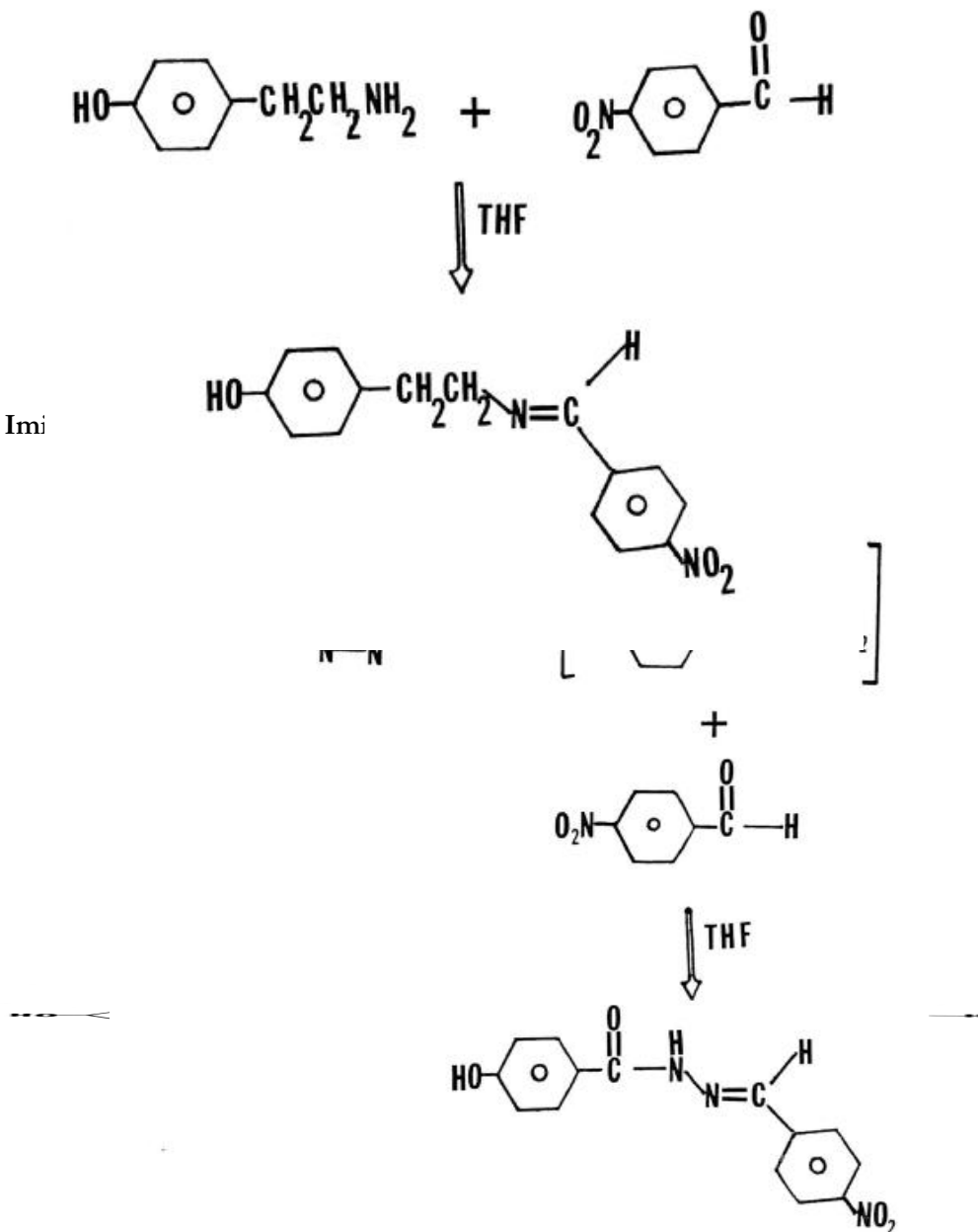
Scheme 3 (The Hydrazone)
