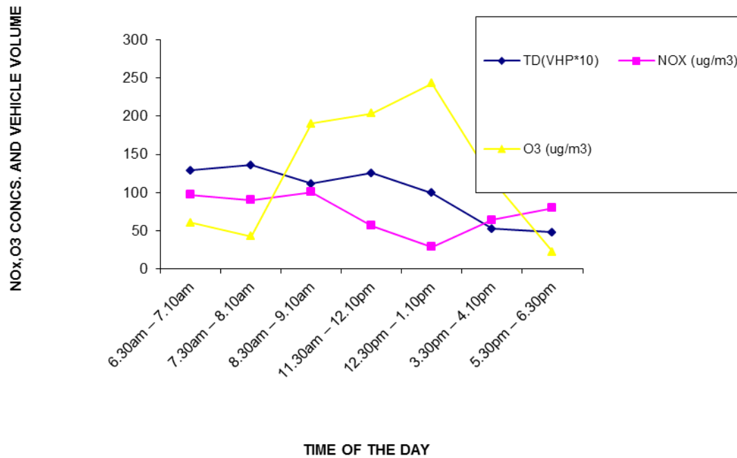
Figure 3: Diurnal Variation of Traffic Density with Trace Gas Concentrations for IA-LT Sites appear to have low values in the morning but increases gradually during the day reaching a peak in the mid-afternoon before eventual gradual decrease to minimum values in the evening.
