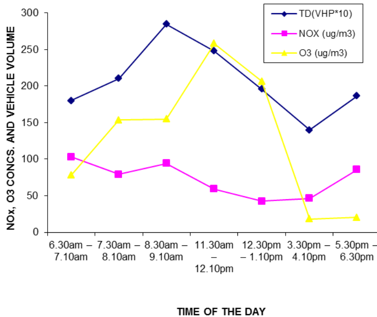
Figure 1: Diurnal Variation of Traffic Density with Trace Gas Concentrations for HT-MPD Sites
