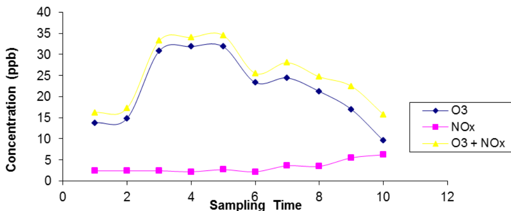
Figure 4: Mean Daily Mixing Ratios of O 3 , NO x and O 3 +NO x of Ilorin Town during Rainy Season
