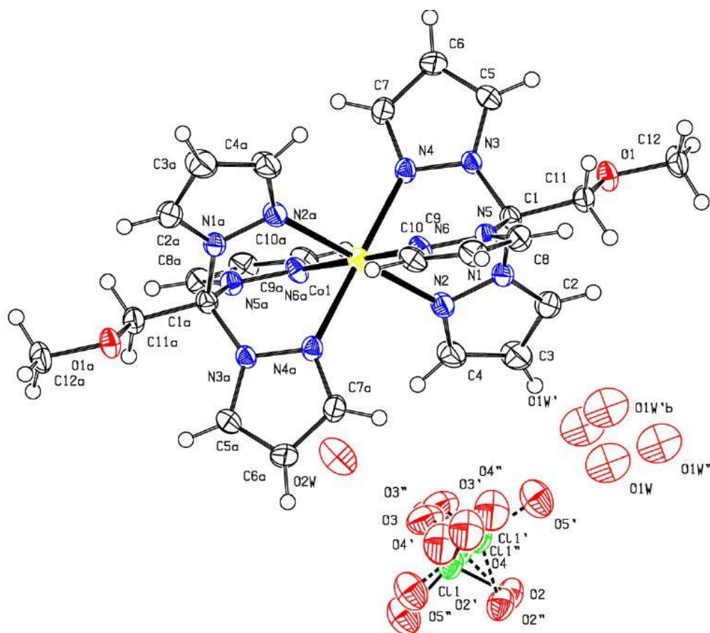
Figure 2. View of molecular structure of bis[1-methoxy-2,2,2-tris-(pyrazol-1-yl- \kappa N 2 ) ethane]-cobalt (II) bis-perchlorate, with atom labeling. Displacement ellipsoids are drawn at the 50% probability level.
